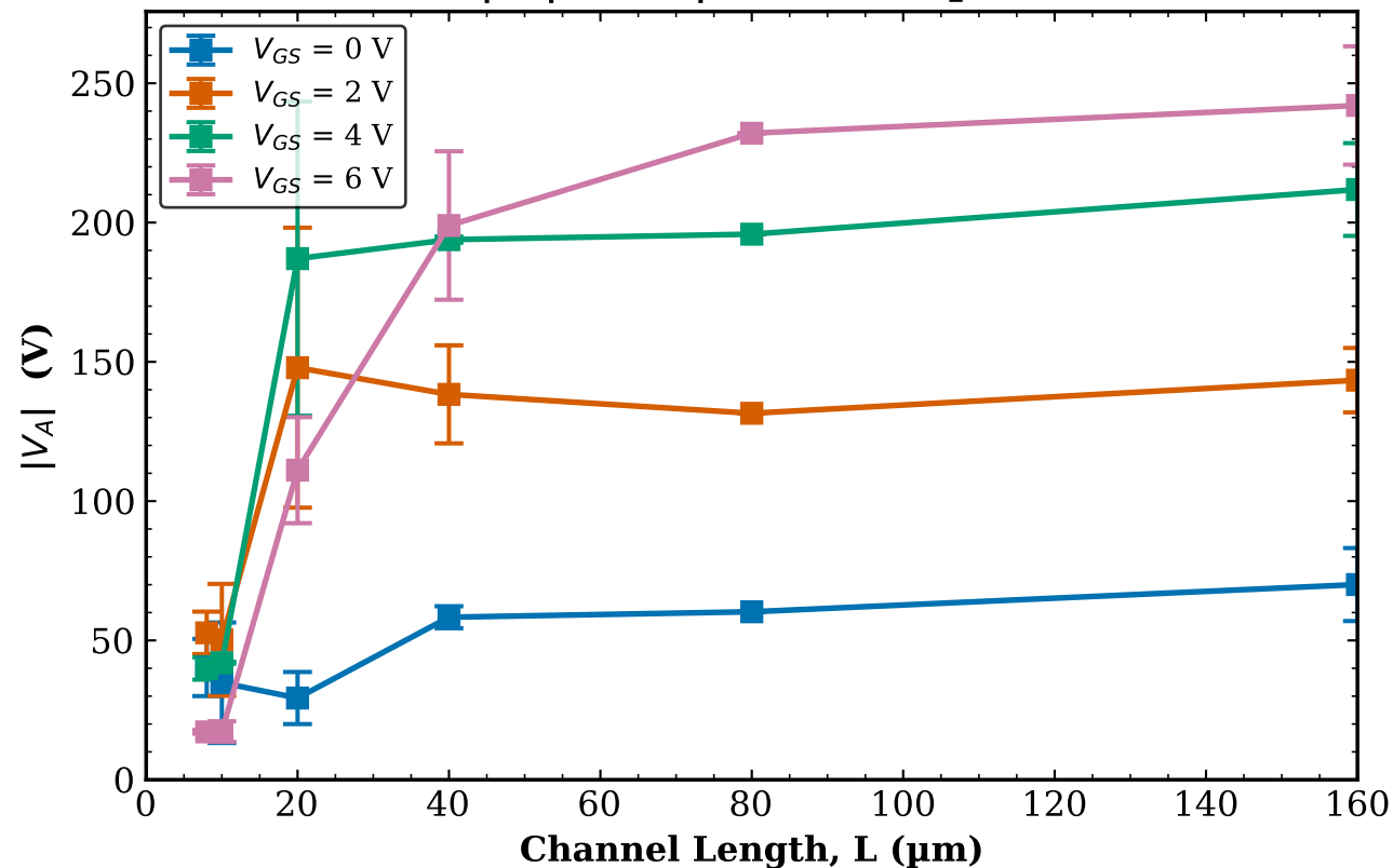
TFT1 Combined (Tr. 1 & 2) |V_A| vs L | W = 100\text{ }\mu\text{m}
